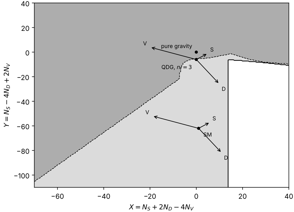
Figure 1: Existence of an admissible fixed point in the (X, Y) plane (optimised cutoff, scheme B). Light grey: fixed point exists but is outside the range g_* < 2 , \lambda_* > -1 ; dark grey: exists and is inside that range; white: no admissible fixed point. Arrows: displacement by five hidden massless vectors (V), real scalars (S) or Dirac fermions (D), starting from QDG-like content with n_f = 3 and from the Standard Model. Script hs_figure.py .
